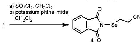
Scheme 2. Preparation of Se -Cyanoethylphthalimide 4
