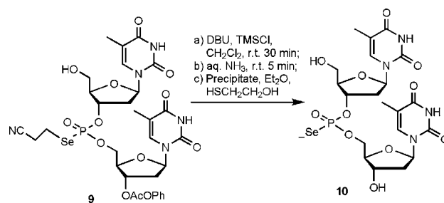
Scheme 4. Unblocking of Dinucleotide Se -(2-Cyanoethyl) Phosphoroselenoate Triester 9
