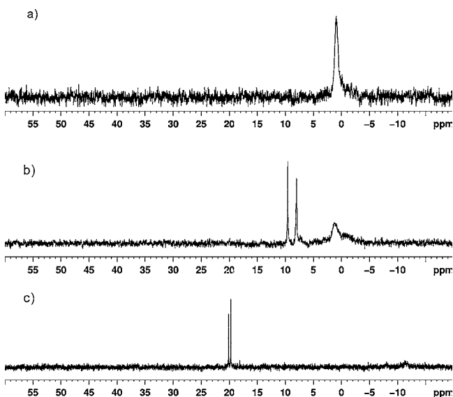
Figure 1. ^{31}\text{P} NMR spectra of the reaction described in Scheme 3: (a) H-phosphonate 5 ; (b) 5 and 6 in the presence of pivaloyl chloride (step a); and (c) after addition of selenium transfer reagent 1 (step b).
