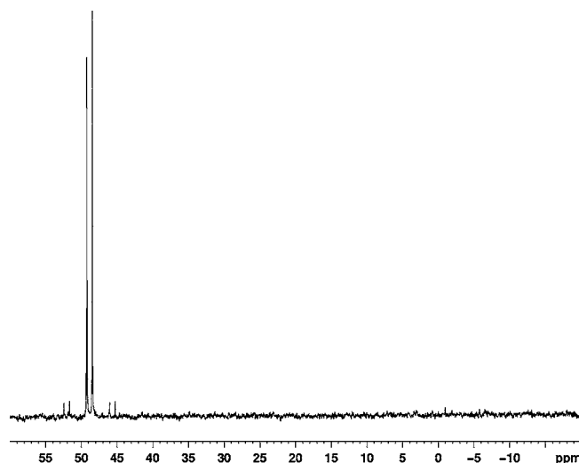
Figure 4. ^{31}\text{P} NMR spectrum of phosphoroselenoate diester 10 .
