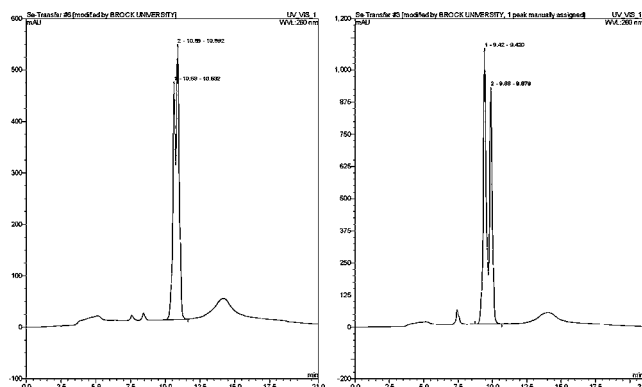
Figure 5. C18 HPLC profiles on 10 (left) and 12 (right). See the Supporting Information for the eluting program.
