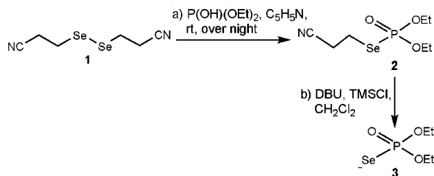
Scheme 1. Reaction of Diethylphosphite with Se -(2-Cyanoethyl)diselenide 1
