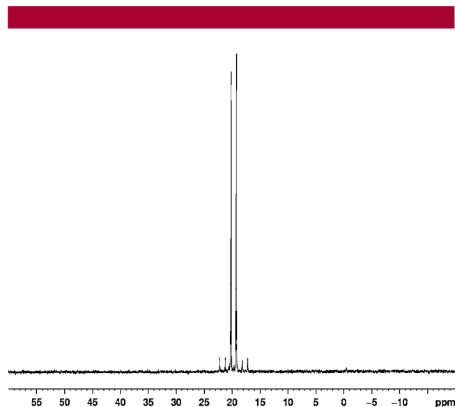
Figure 2. ^{31}\text{P} NMR spectrum of Se -(2-cyanoethyl) phosphoroselenoate triester 9 .
