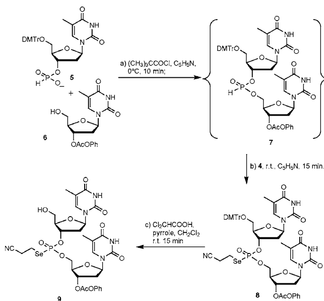
Scheme 3. Synthesis of Se -(2-Cyanoethyl) Phosphoroselenoate Triester
