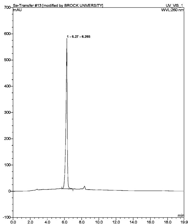
Figure 3. \text{C}_{18} HPLC profile of triester 9 (see the Supporting Information for the eluting program).
