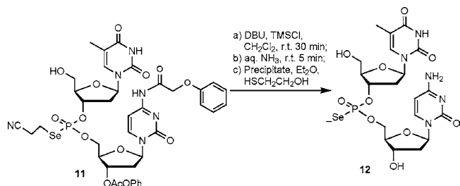
Scheme 5. Unblocking of Tp(Se)C Dimer Phosphoroselenoate 11
